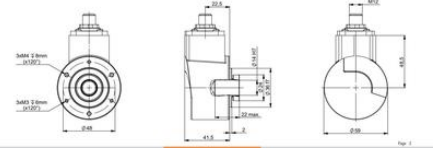
THK5_14, Connection BFR (Radial M12)
