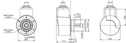
THM5_10, Connection BJA (Axial cable)
