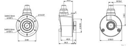
AH05S14/DM/ Flange side clamping, Connection BFR (Radial M12)
