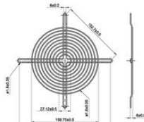
MG-18 (For UF18JC Series) *Steel
