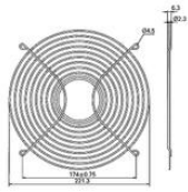
MG-25 (For UF25HC, 25GC, 25GCA, 25GCB, 25JC Series) *Steel
