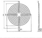
MG-15 (For UF15P, 17P, 15PC, 15KC, 17PC, 15AC Series) *Steel
