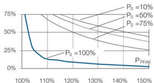
Operating characteristics
