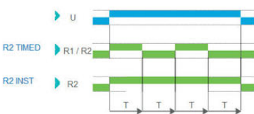
Function Di - Symmetrical flashing (ON Start)
