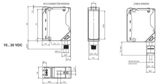
DC MODELS
